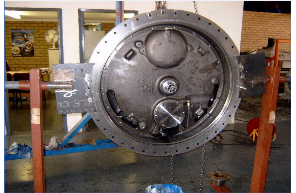
Disassembling a YK York Compressor
