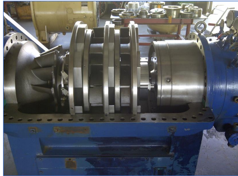
Assembling York Multi Stage Comp
